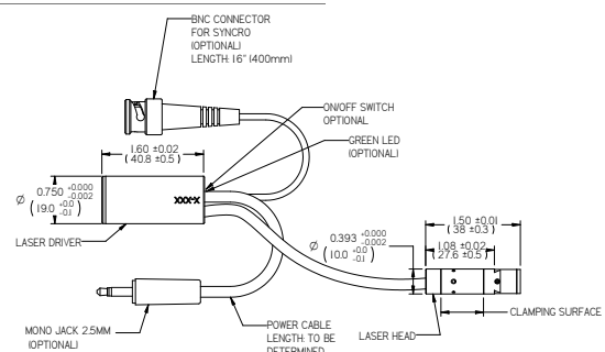
MINI LASER WITH SEPARATE ELECTRONICS OPTION
