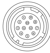
HIROSE HR10A-10R-12PB-01
